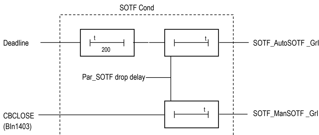
Figure 3-2 The scheme of the “switch-onto-fault” preparation
